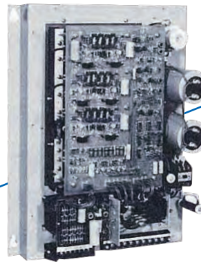
VS-616T (1974) Transistor AC drive
